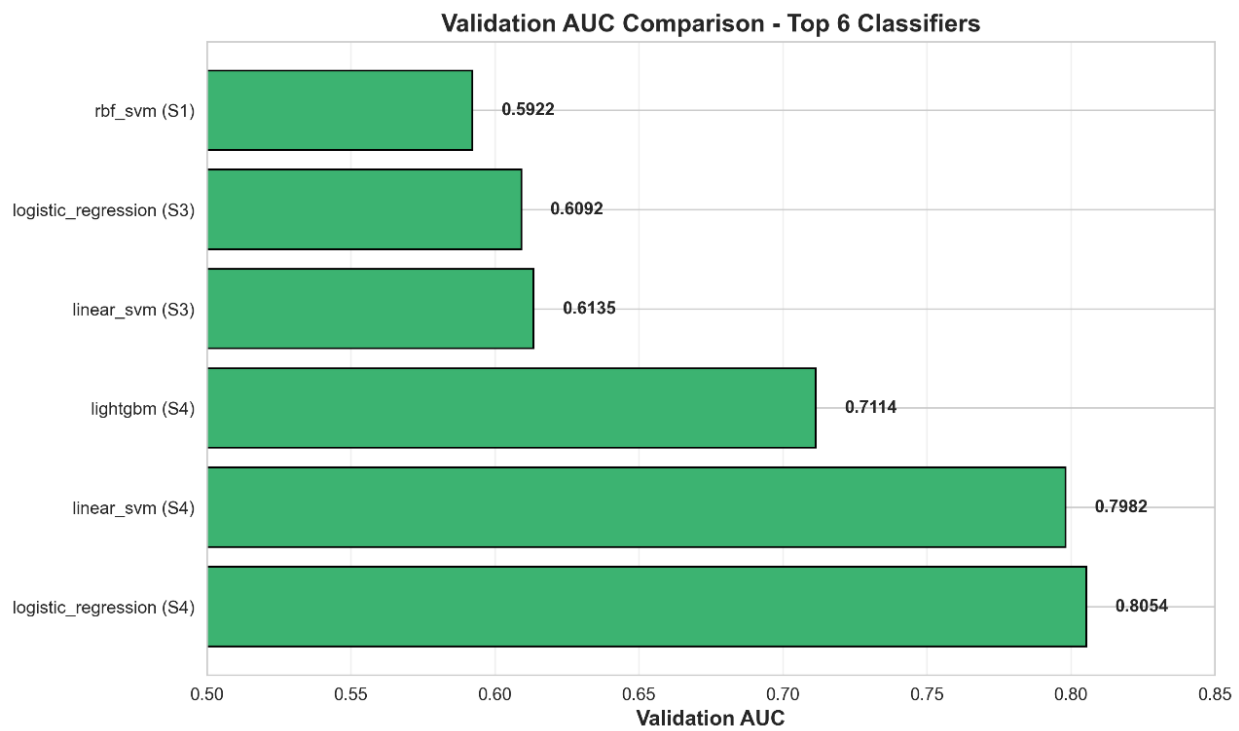
Figure 5.2 :AUC for Different Classifiers.
