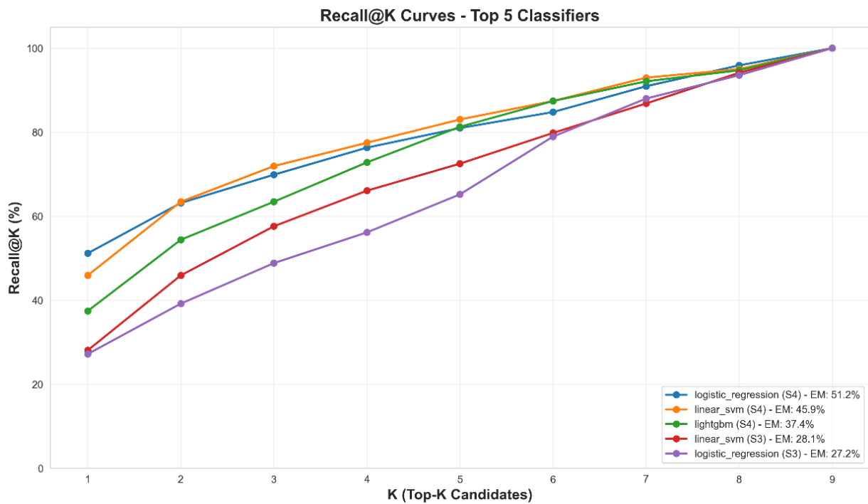
Figure 5.3 : Recall@K Curves for the Top Five Meta-Classifiers.
