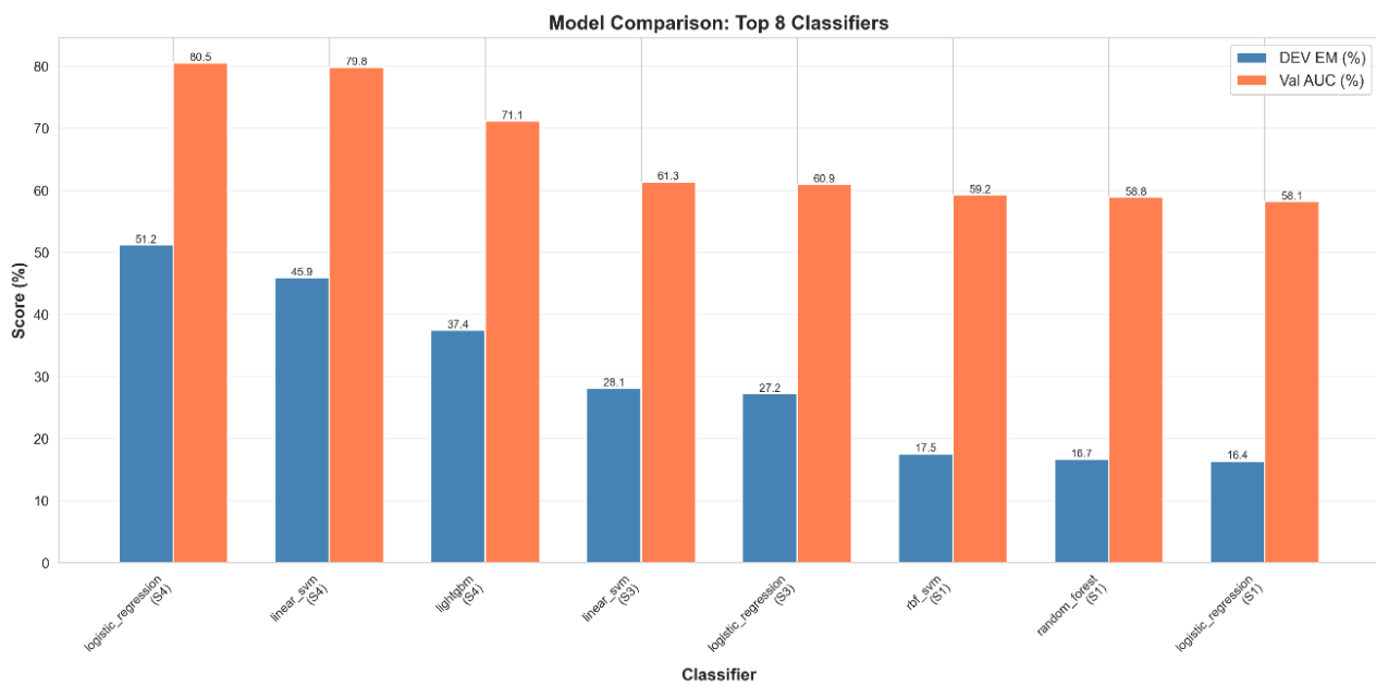
Figure 5.4 :DEV EM and Val AUC Values for Eight Classifiers.
