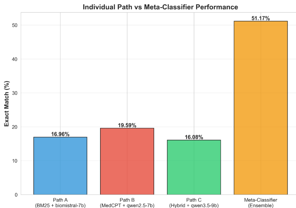
Figure 5.1 :Performance of Individual Pathways versus the Meta-Classifier.
