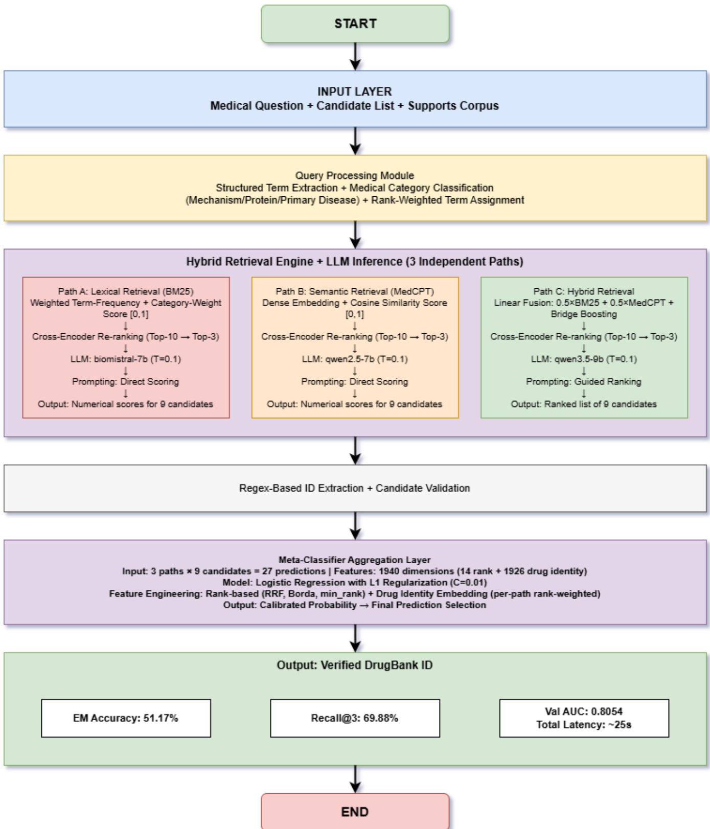
Figure 4.1: Optimal Multi-Path Ensemble Architecture for Multi-Hop Biomedical Reasoning.
