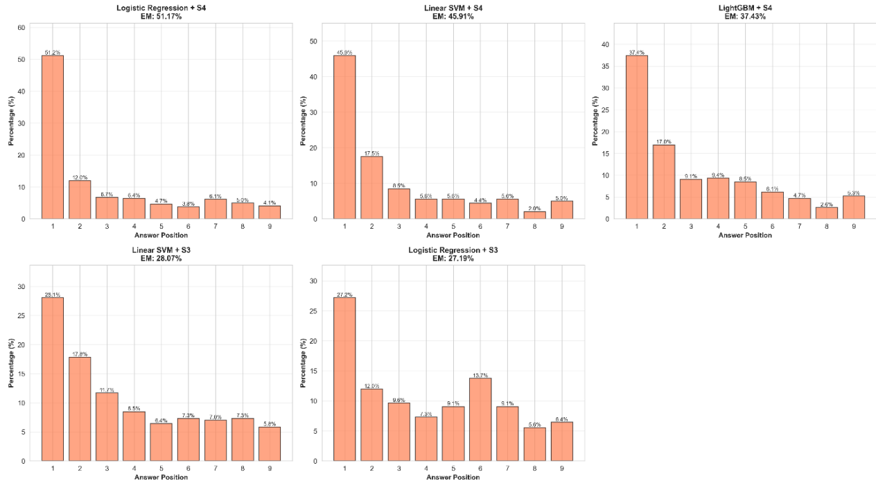
Figure 5.5 :Distribution of Correct Answers.
